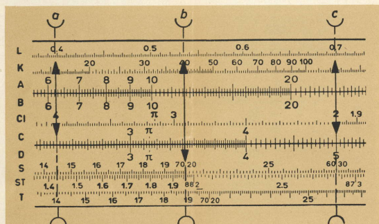
Fig. 23 Briggse logarithmen (grondtal 10) a) \lg 2.5 = 0.3980 b) \lg \sin 20^\circ = 9.5340 - 10 c) \text{num } \lg 1.6990 = 50
