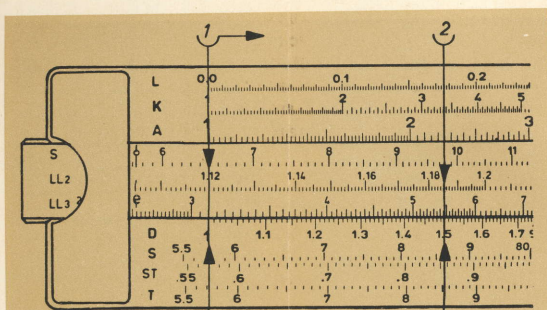
Fig. 26 q^n = \left(1 + \frac{p}{100}\right)^n = \left(1 + \frac{12}{100}\right)^{1.5} = 1.12^{1.5} = 1.185
