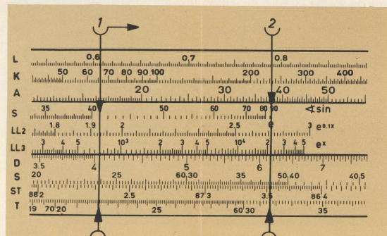
Fig. 30 \tan \beta = \frac{\tan 22^\circ}{\sin 41^\circ} \beta = 31.6^\circ
